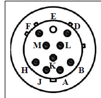
Harness Connector Pin View
